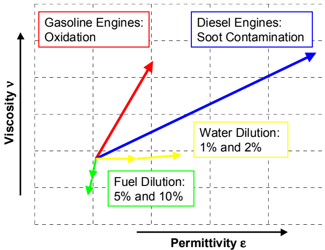
Figure 4: Correlation of oil condition with sensor measurements
